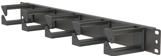
1U 19" Modular Cable Organizer | With 5 Snap In Rings
