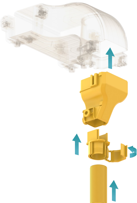
Reducer to Flex Tube Assembly
