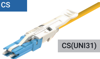
Standard CS Duplex Connector
